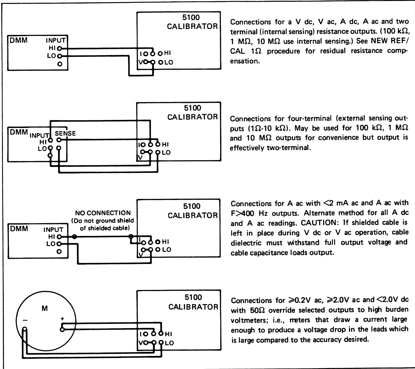
Figure 2-12. Meter Connections
