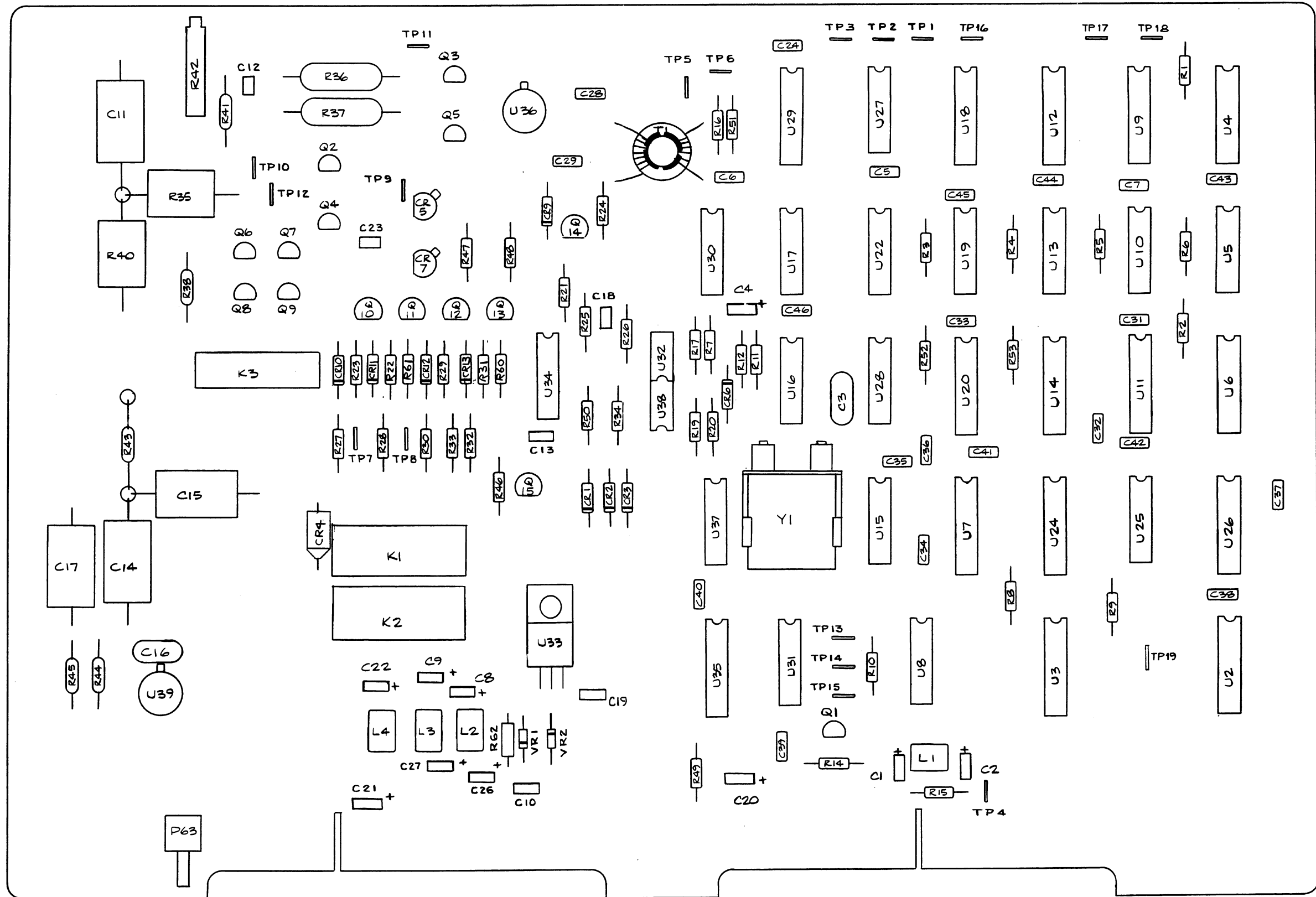
Figure 7-13. A15 Digital-to-Analog PCA
