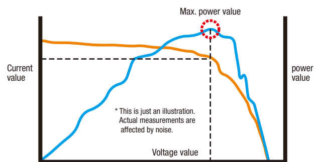
Typical voltage, current, and power measurements in MPPT control
