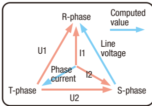
Figure 1 Line voltage/phase current
