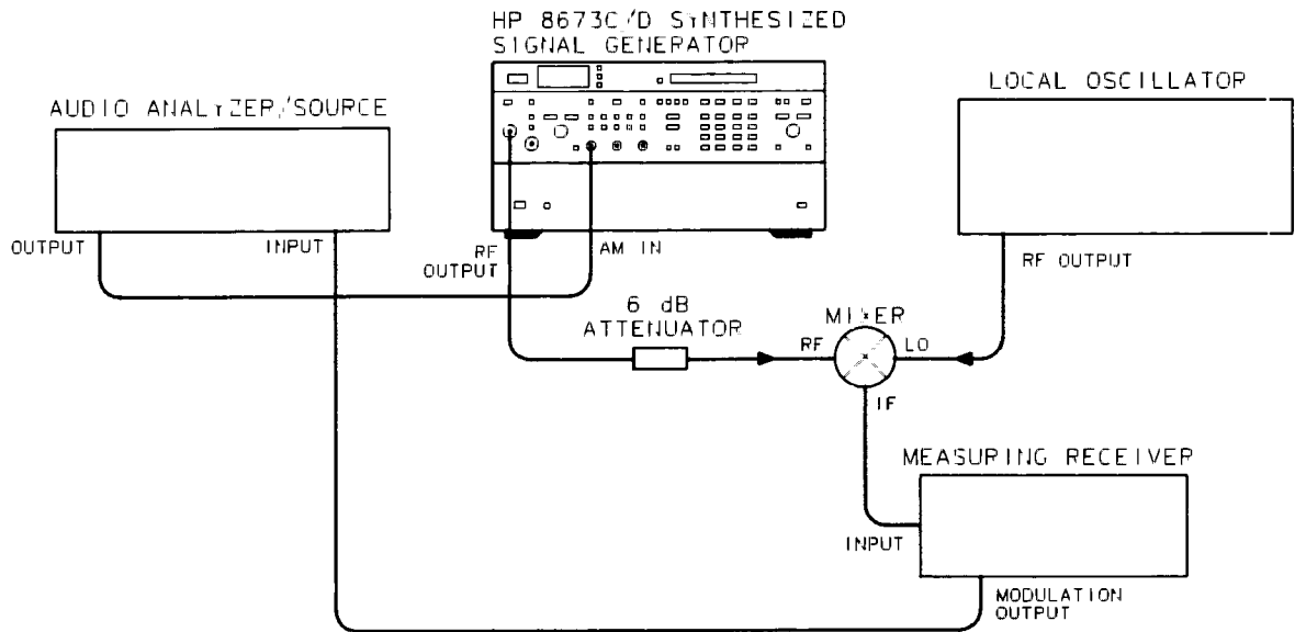
Figure 4-32. AM Bandwidth Test Setup
