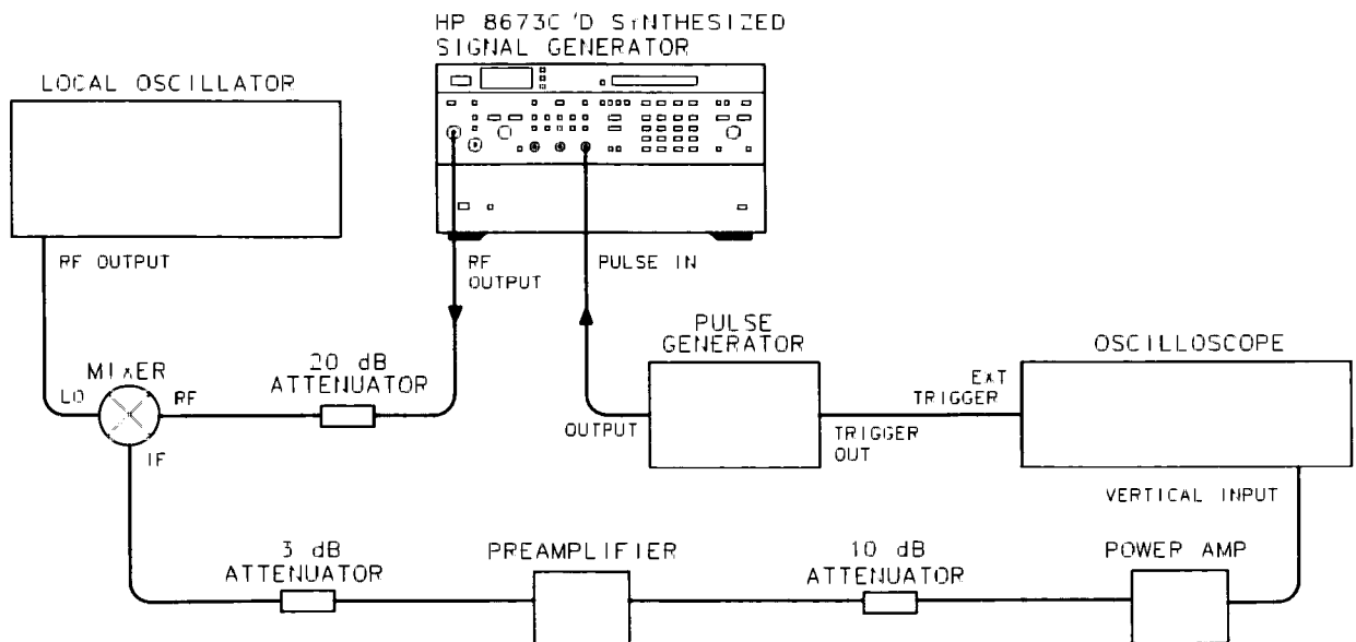
Figure 4-30. Pulse Peak Level Accuracy Test Setup
