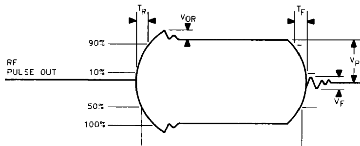
Figure 4-29. Pulse Definitions
