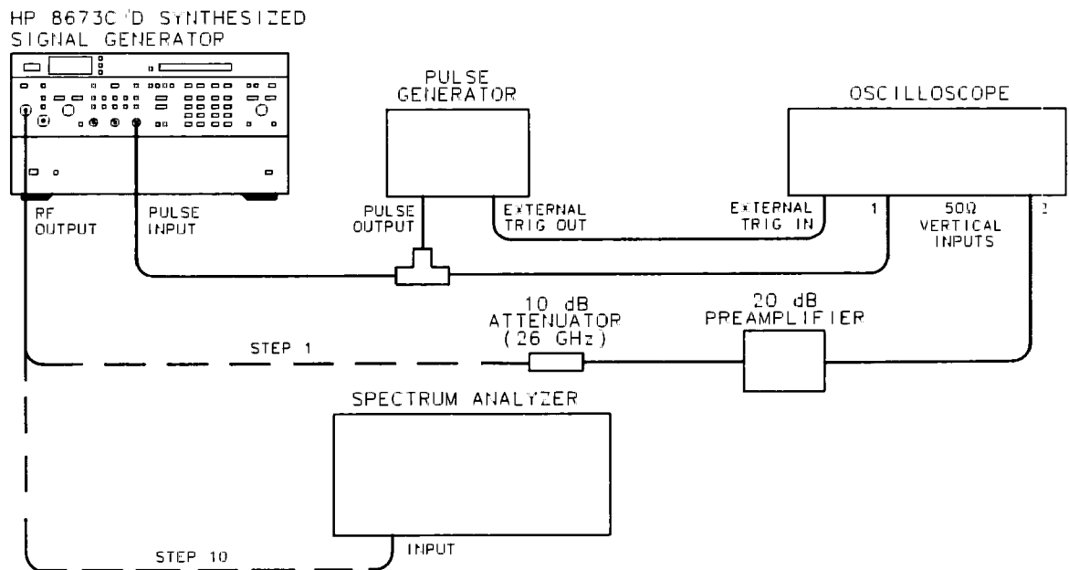
Figure 4-4. Low Frequency Pulse Test Setup
