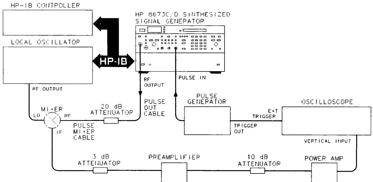
Figure 4-27. Pulse Rise/Fall Time and Overshoot Test Setup
