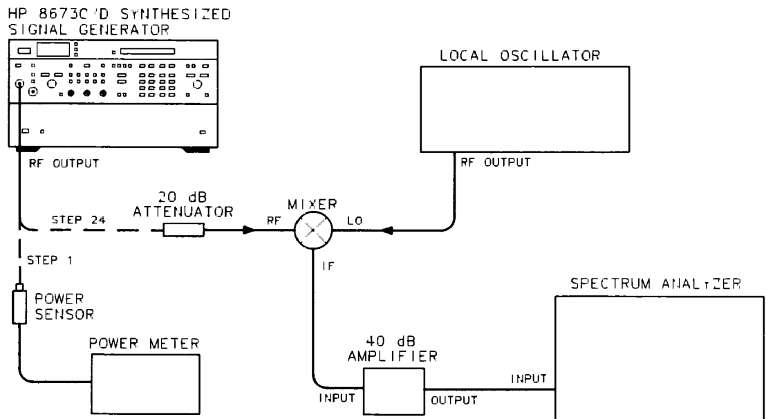
Figure 4-22. Absolute Level Accuracy Test Setup
