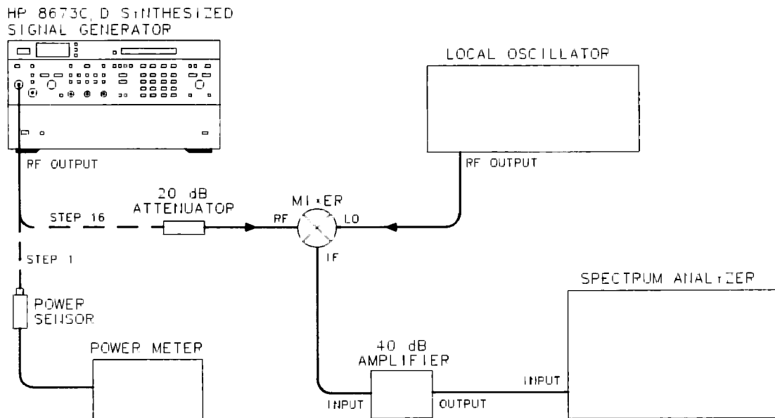
Figure 4-3. Level Accuracy Test Setup
