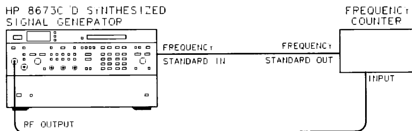
Figure 4-1. Frequency Range and Resolution Test Setup
