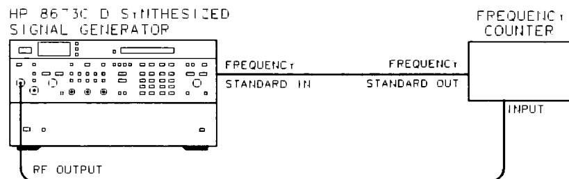
Figure 4-10. Frequency Range and Resolution Test Setup
