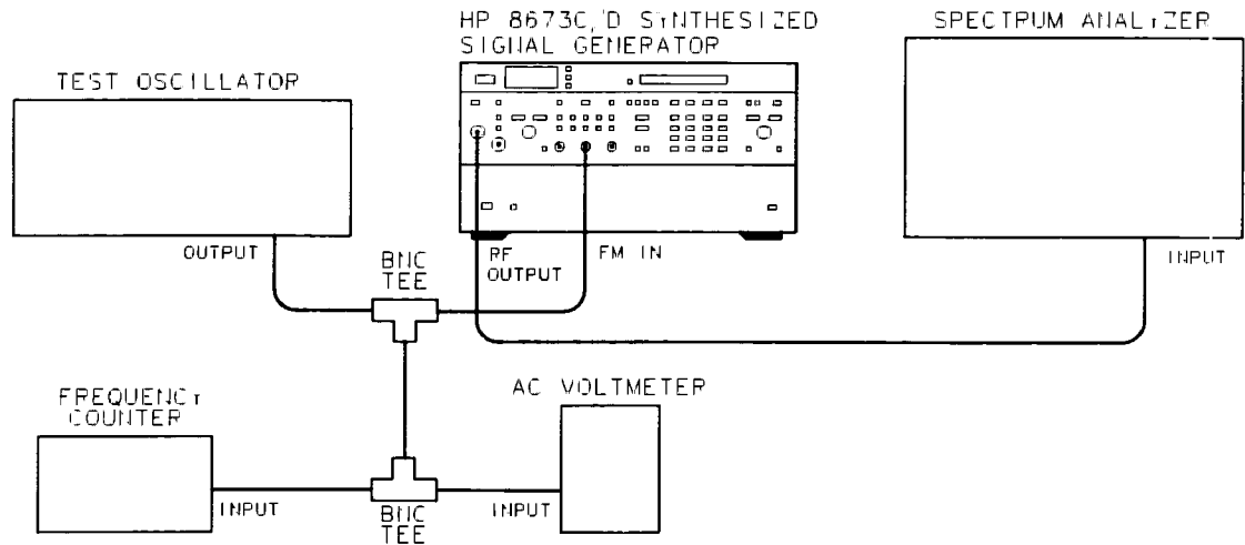
Figure 4-36. FM Frequency Response Test Setup
