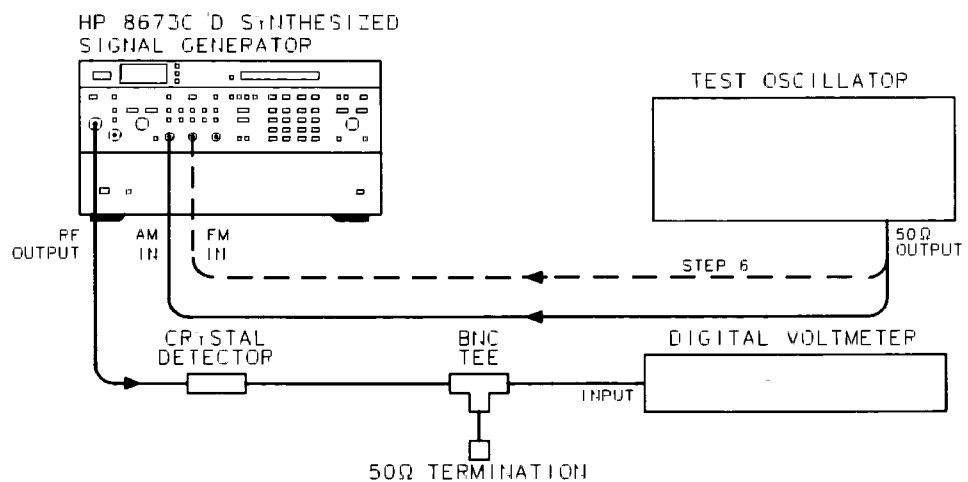
Figure 4-38. Incidental AM Test Setup
