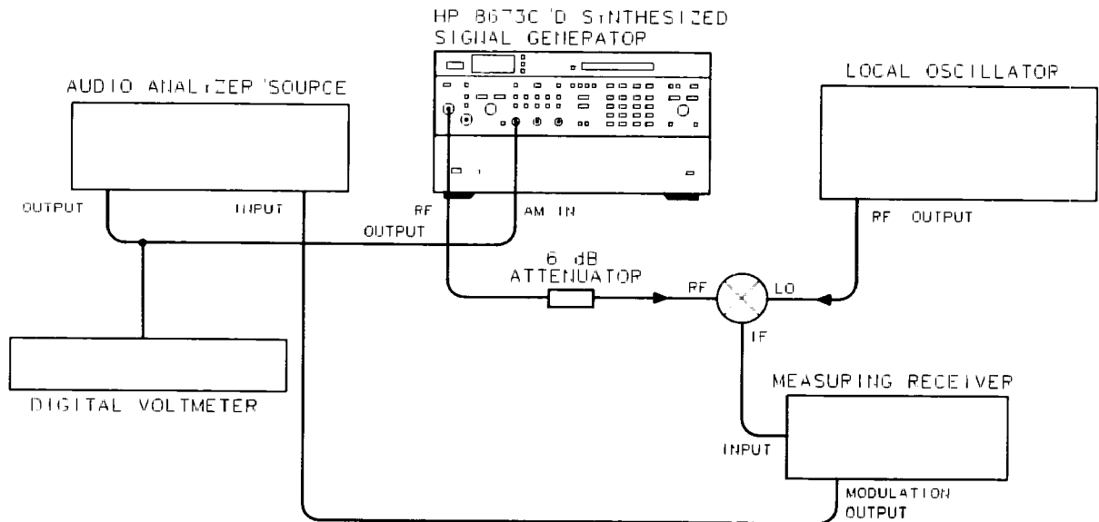
Figure 4-35. Incidental FM Test Setup, Part Two.
