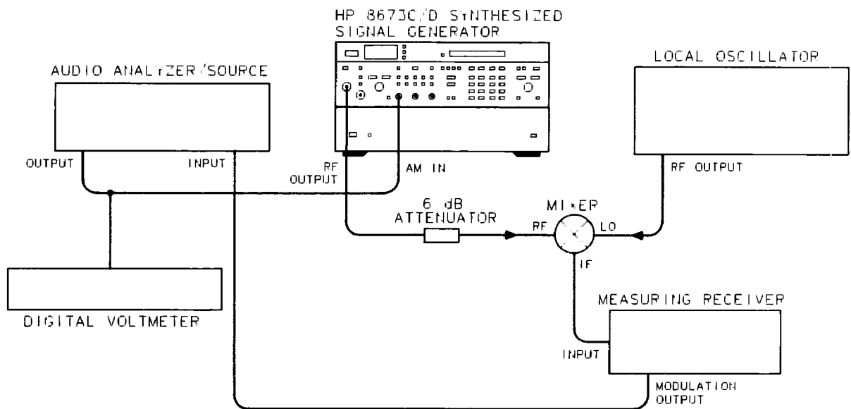
Figure 4-8. AM Accuracy Test Setup
