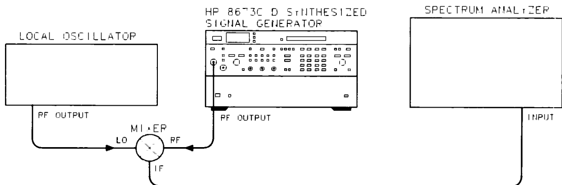
Figure 4-17. Single-Sideband Phase Noise Test Setup
