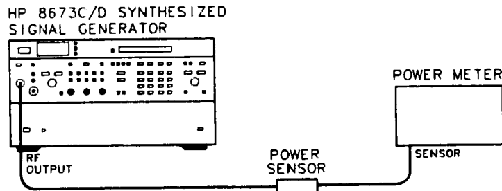
Figure 4-2. Output Level and Flatness Test Setup
