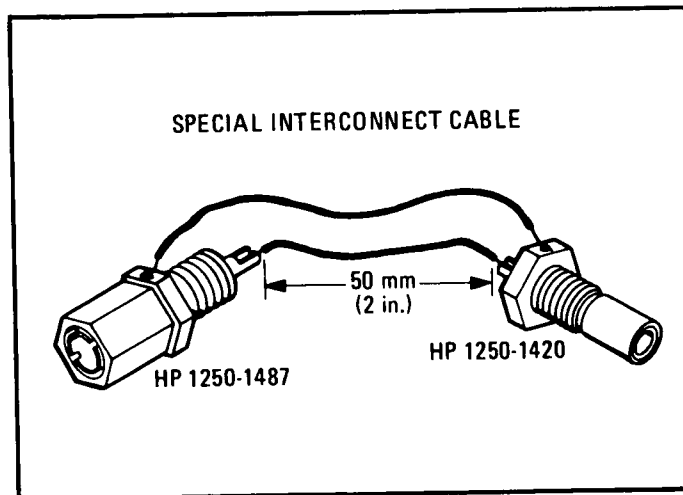
Figure 1-2. Special Interconnect Cable
