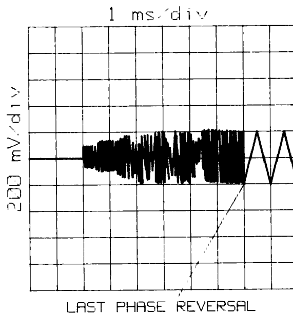
Figure 4-14. Frequency Switching Time Measurement Waveform
