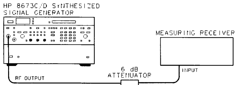
Figure 4-34. Incidental FM Test Setup, Part One
