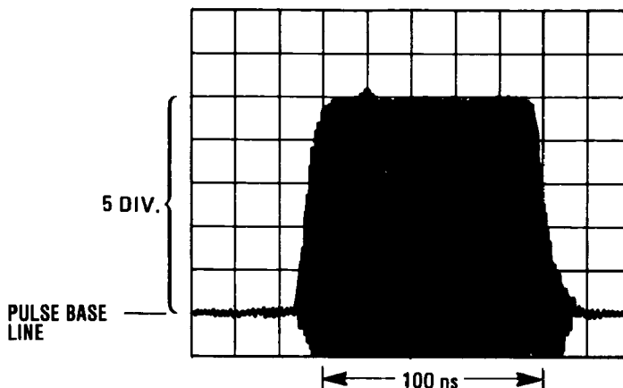
Figure 4-5. Risetime, Overshoot and Ringing Measurement
