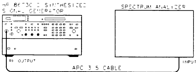
Figure 4-19. Non-harmonically Related Spurious Test Setup
