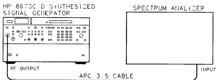
Figure 4-26. Pulse ON/OFF Ratio Test Setup
