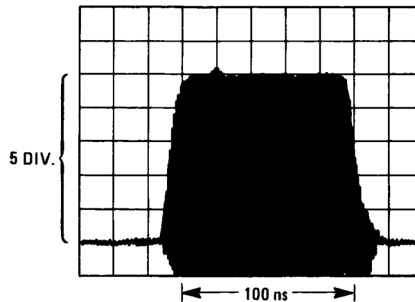
Figure 4-28. Pulse Rise/Fall Time and Overshoot Waveform
