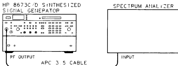
Figure 4-18. Harmonics, Subharmonics, and Multiples Test Setup
