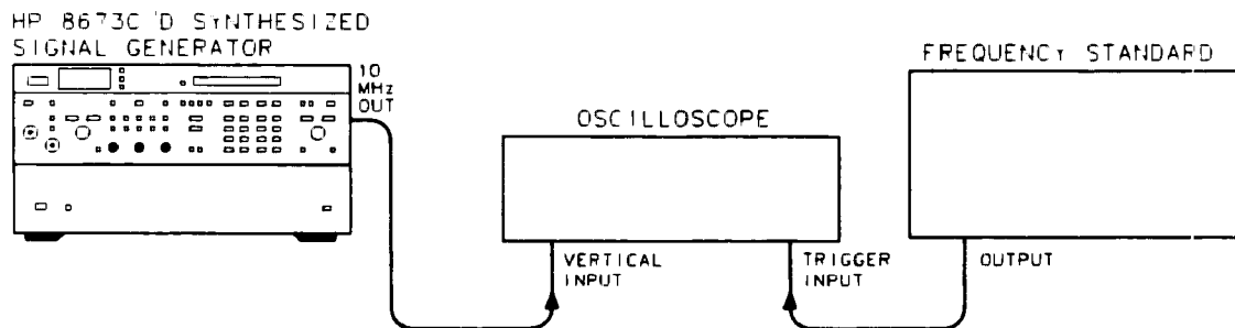
Figure 4-11. Internal Time Base Aging Rate Test Setup
