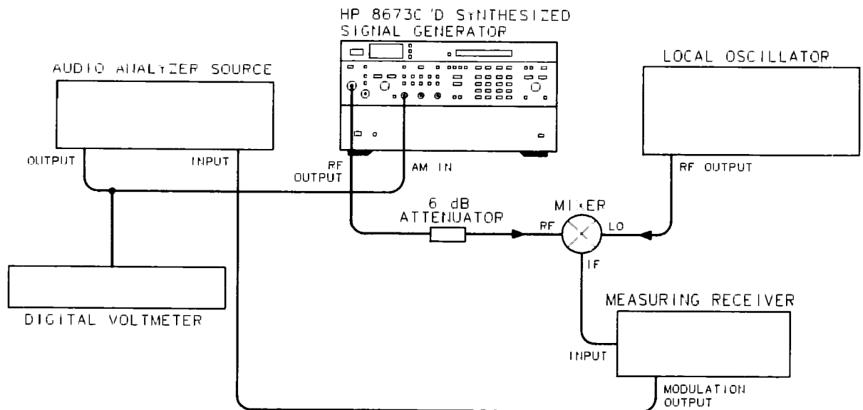
Figure 4-33. AM Accuracy Test Setup
