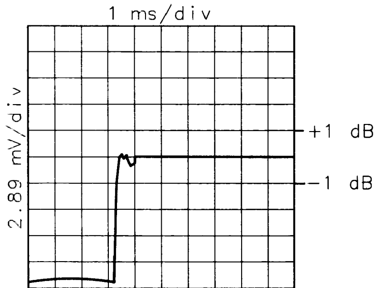
Figure 4-25. Level Switching Time Measurement Waveform
