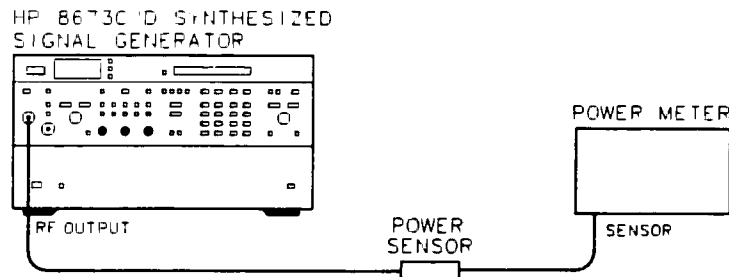
Figure 4-21. Output Level and Flatness Test Setup
