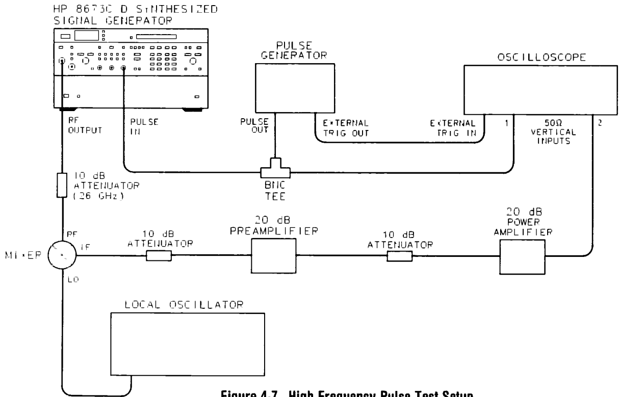
Figure 4-7. High Frequency Pulse Test Setup
