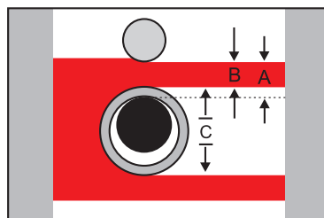
Step 2: Place product on mandrel and take measurements Wall = A - B OD = C ID = OD - (2 \times Wall)
