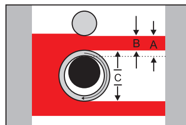
Step 3: Rotate the product to attain multiple points of measurement as well as concentricity and ovality Concentricity = \Delta (A - B) Ovality = \Delta C
