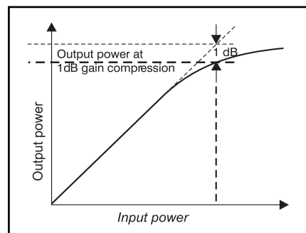
Output power variation against input power showing amplifier going into compression.
