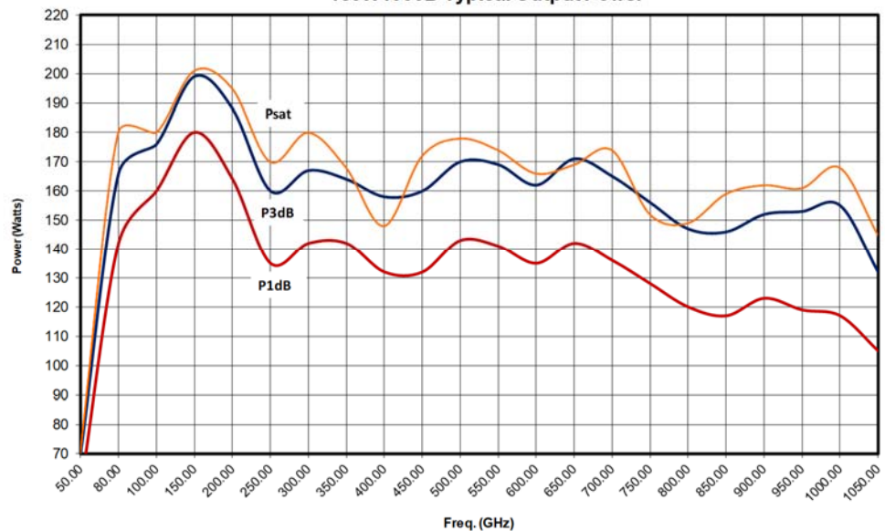
150W1000B Typical Output Power
