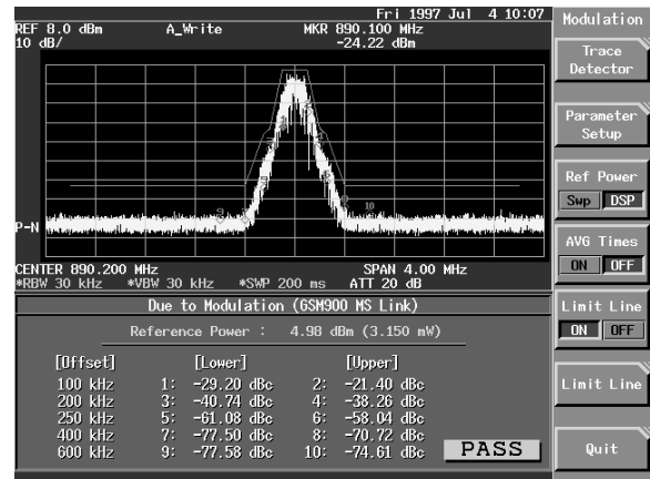
▲ Modulation spectrum measurement
