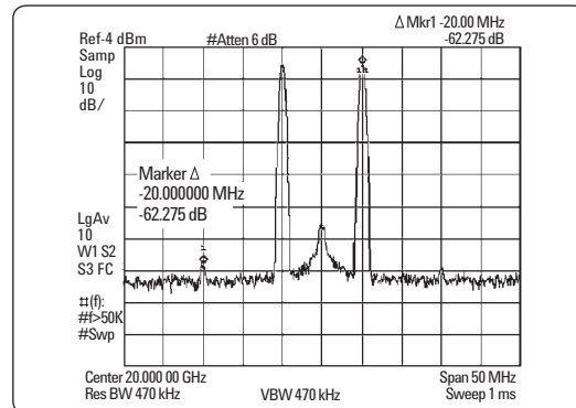
20 GHz two tone (measured)
