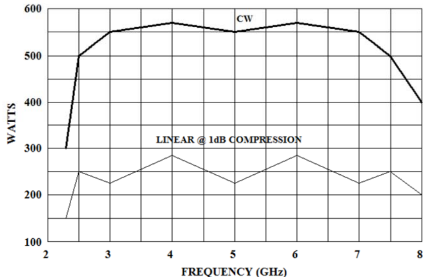
500T2G8 TYPICAL POWER OUTPUT
