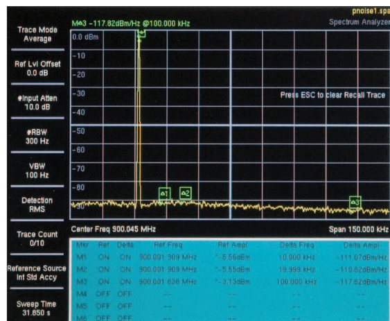
Phase Noise
