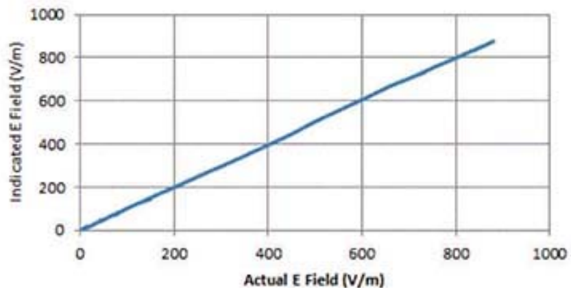
Linearity Response at 1 GHz
