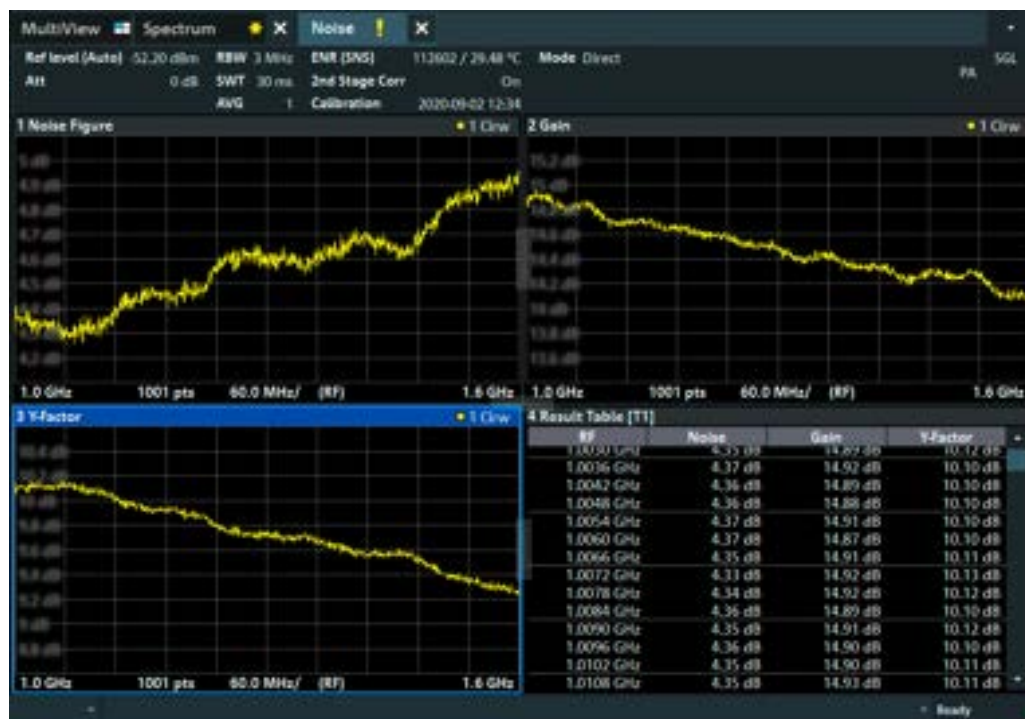
Simultaneous view of graphs for noise figure, gain and Y-factor versus frequency and a table of the results in numerical format
