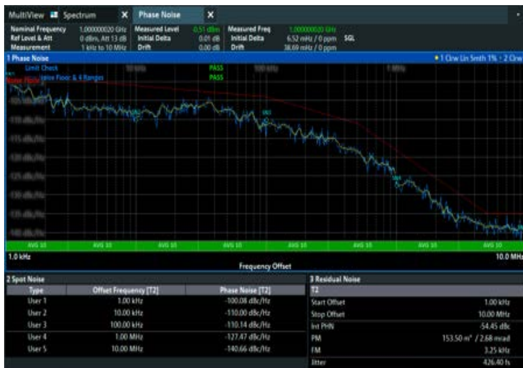
Phase noise measurement plus automatic limit checking, spot noise and residual noise indication
