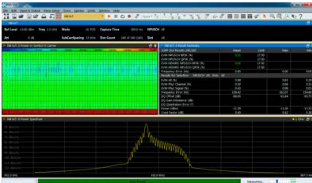
Demodulation and EVM measurement of an NB-IoT UL signal with the R&S®VSE-K106 measurement application
