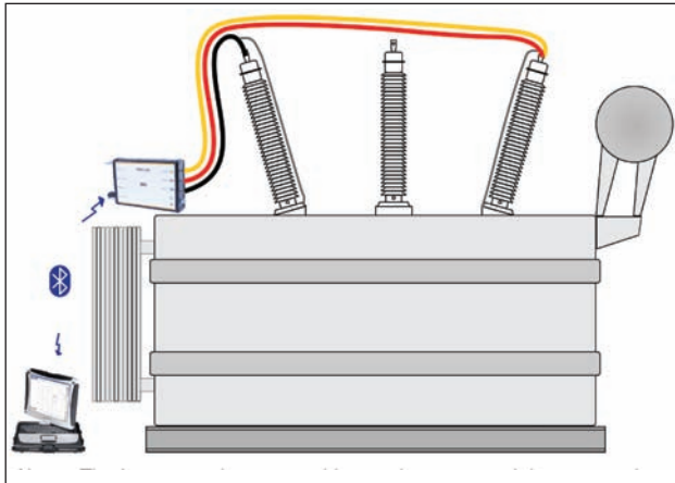
The laptop can be operated by touch screen and the communication is wireless via Bluetooth. Measurement ground braids connect close to the connection clamps and run next to the bushing to the flange connection to avoid cable loops that otherwise affect the measurement.
