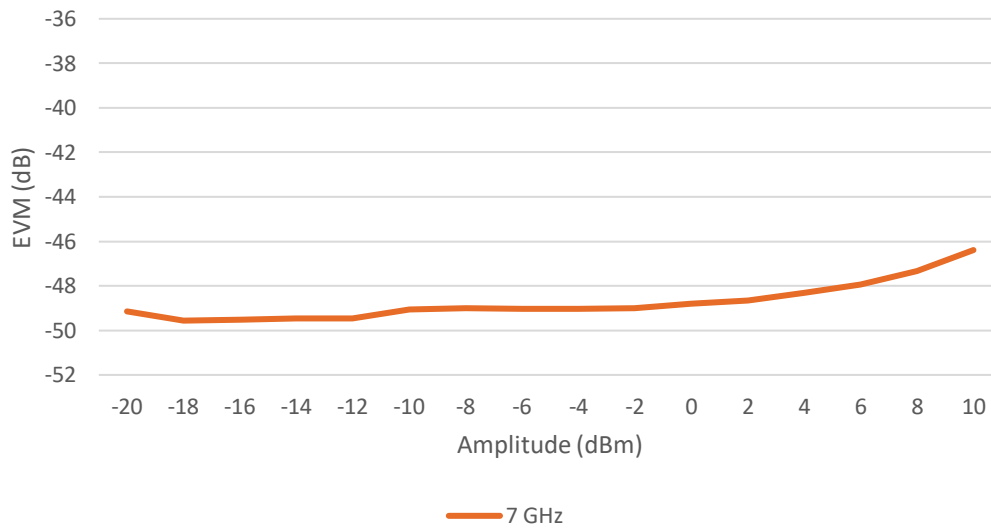
Measured EVM performance vs. power 802.11be, 320 MHz, MCS13
