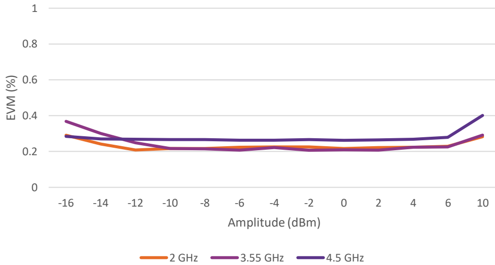
Measured EVM performance vs. power 5G NR, FR1, 100 MHz, SCS60
