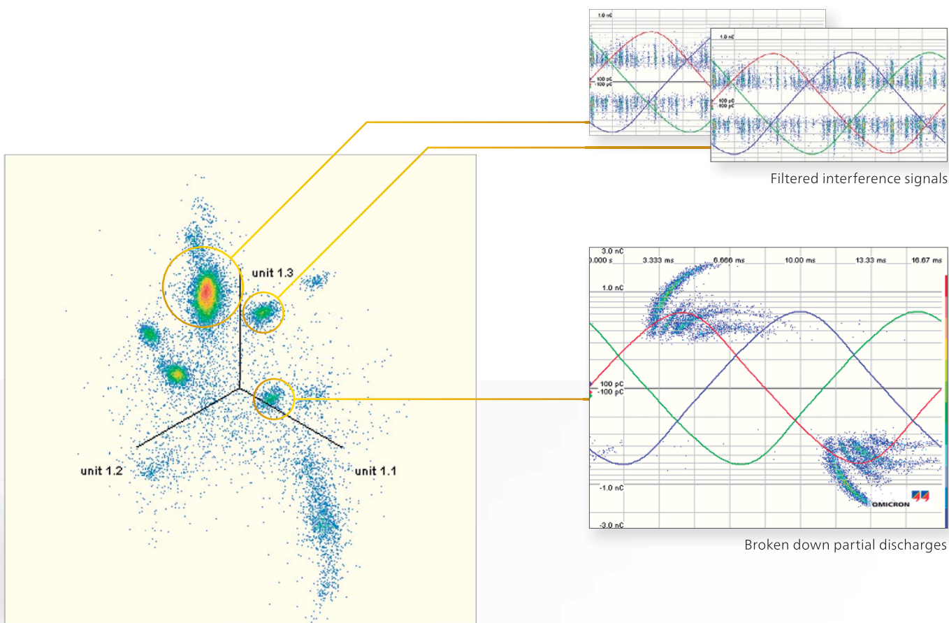
Separation through 3PARD or 3CFRD representation
