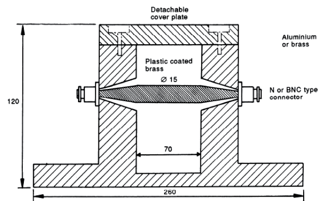
Current Injection Clamp
