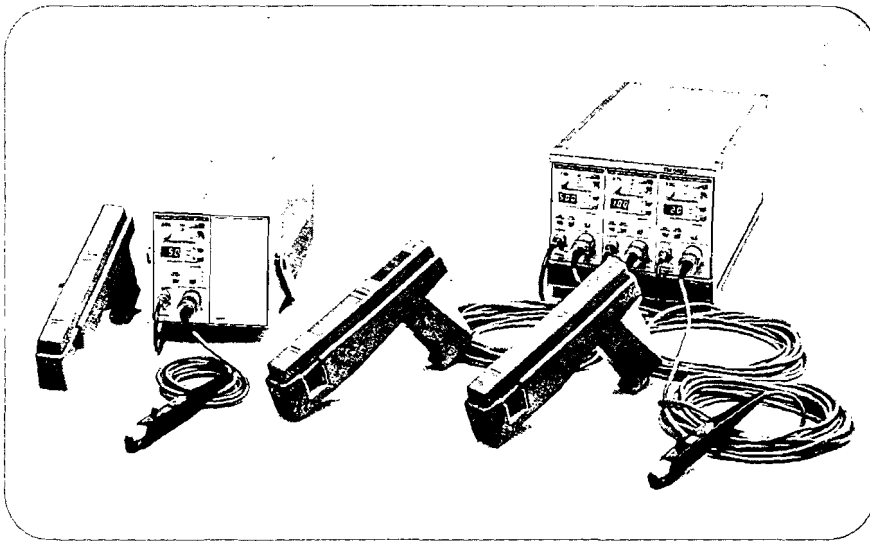
► AM503 Current Measurement Family.
