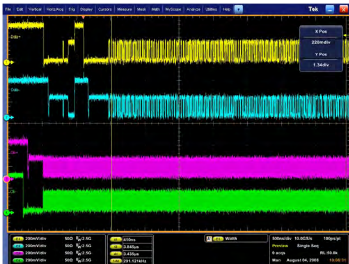
Optional MIPI® D-PHY Characterization and Compliance Testing
