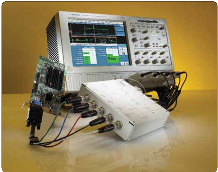
▶ VM5000 with Option VGA – VESA Compliance Test Solution.
