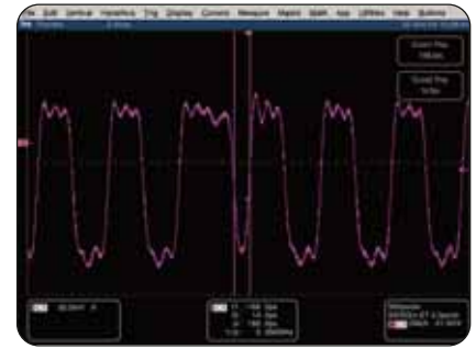
► Trigger on glitches down to 100 ps wide.
