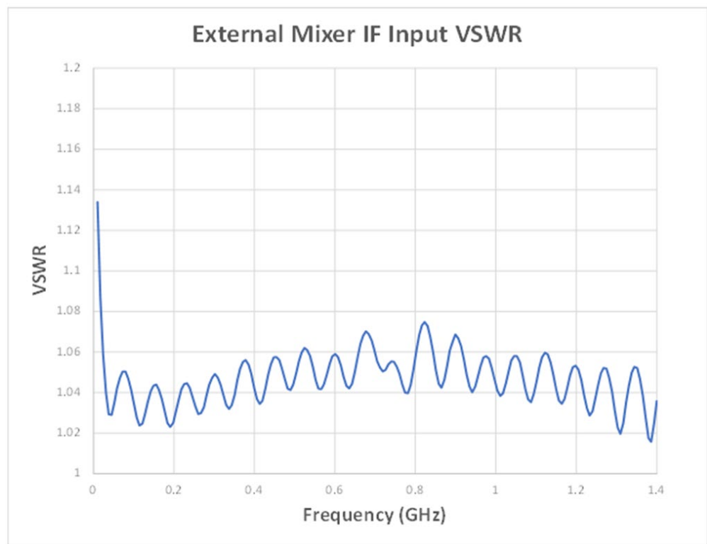
Figure 4. External mixer IF input VSWR
