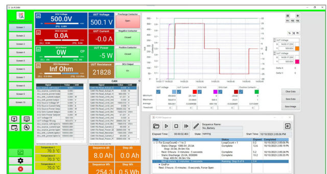
Results display screen showing voltage, current, and the results of a capacity simulation test.
