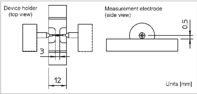
Electrode dimensions
