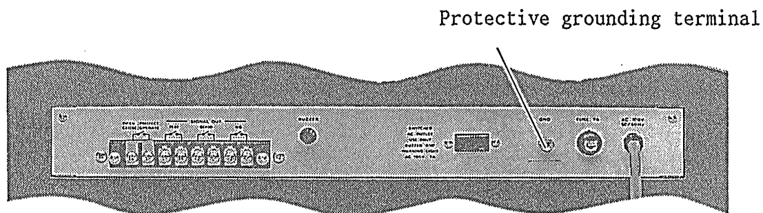
Figure 3.2 Rear of Casing, Model TOS8700
