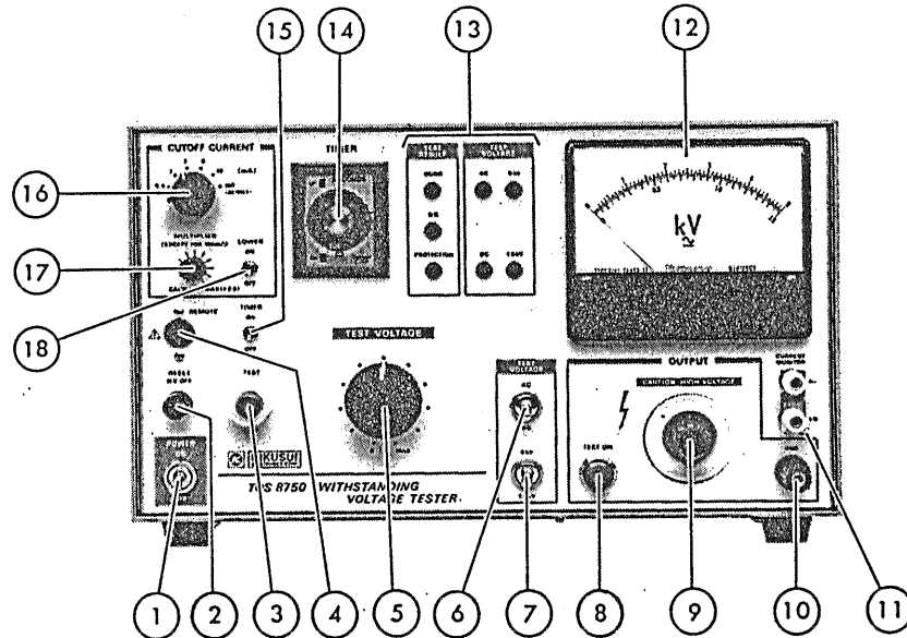
Figure 4.1 Model TOS8750
