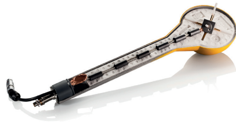
Fig. 3. Internal architecture of a 3-axis antenna. .
