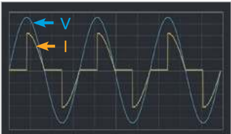
90° Leading Edge Load Waveform
