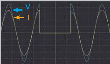
Voltage Interruption Load Testing (CR Mode)
