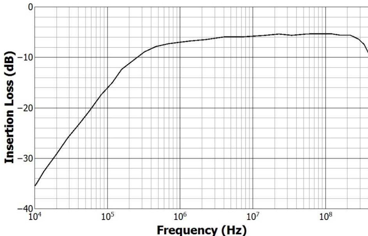
Model 8700i
