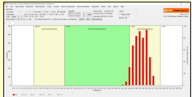
Figure 4: CITRUS - Voltage compliance report as per AS61000.3.100
