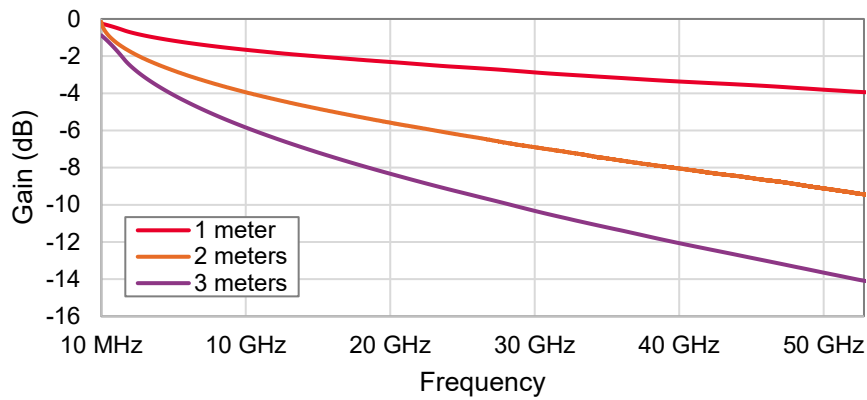
Cable gain (loss) in V3080A bypass path for Keysight cables
