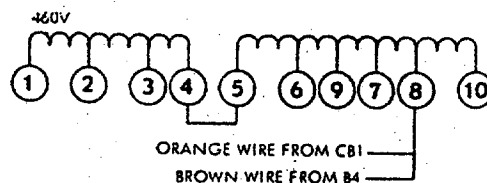
Figure 2-3 Unit Input Connections 20-500, 40-250, 150-70, 300-35, 600-18
