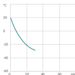
Cool-down time Medium: Ethanol
