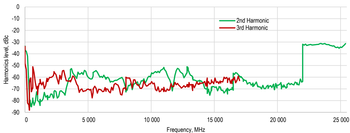
Figure 4. Harmonics at 10 dBm, without option 1EH
