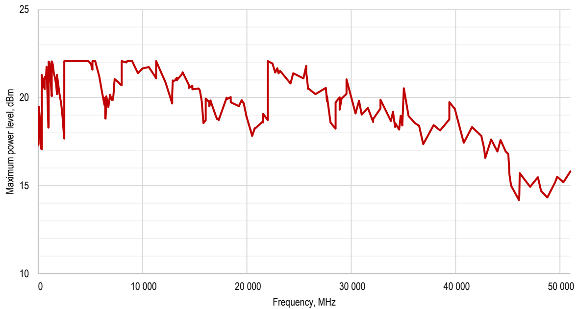
Figure 7. Measured maximum output power, 10 MHz to 51 GHz (Option 2E1)
