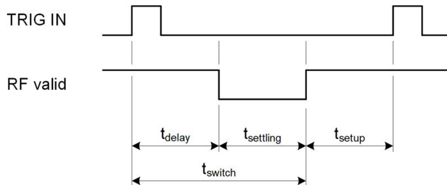
Figure 14. Timing diagram
