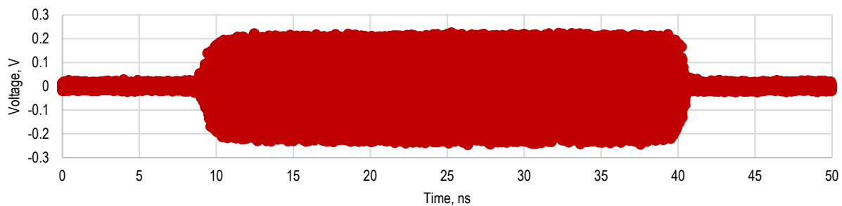
Figure 12. 10 GHz pulse-modulated
