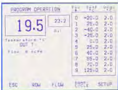
PROGRAM SCREEN
