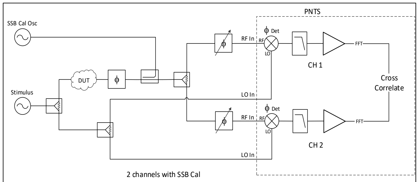
Residual noise measurement of a two-port device using the single-sided spur calibration method
