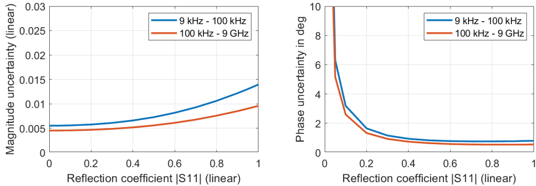
Typical uncertainty of reflection magnitude and reflection phase measurements for the R&S®ZNB3004 with or without frequency upgrade option, in the frequency range from 9 kHz to 9.0 GHz; analysis conditions: S_{12} = S_{21} = 0 , cal. power: -10 dBm, meas. power: -10 dBm
