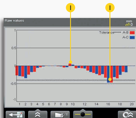
Taper values diagram. Taper out of tolerance (I).
