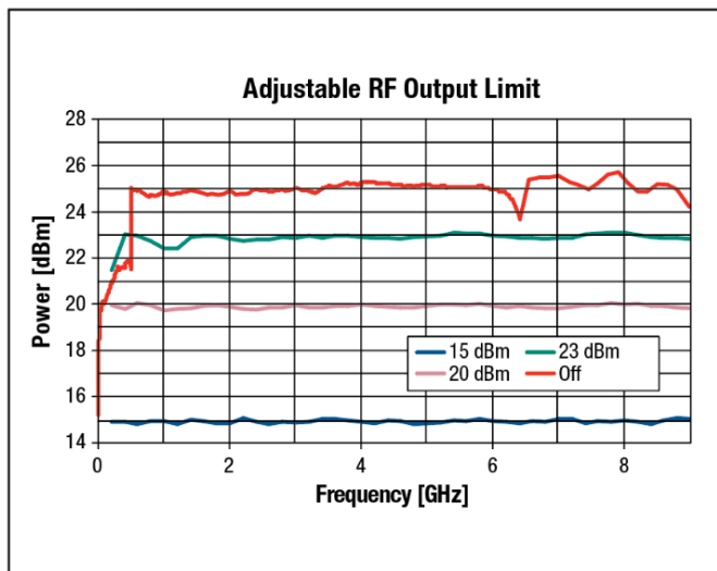
RF output limit (measured)
