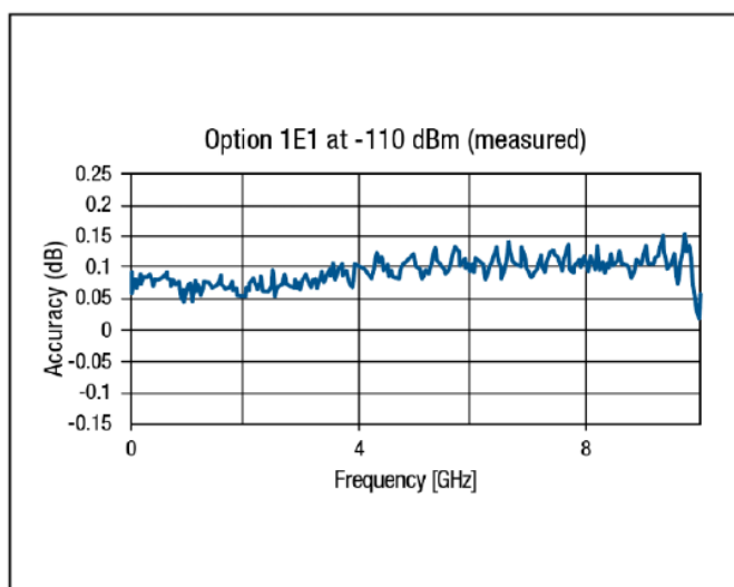
Level accuracy (measured)
