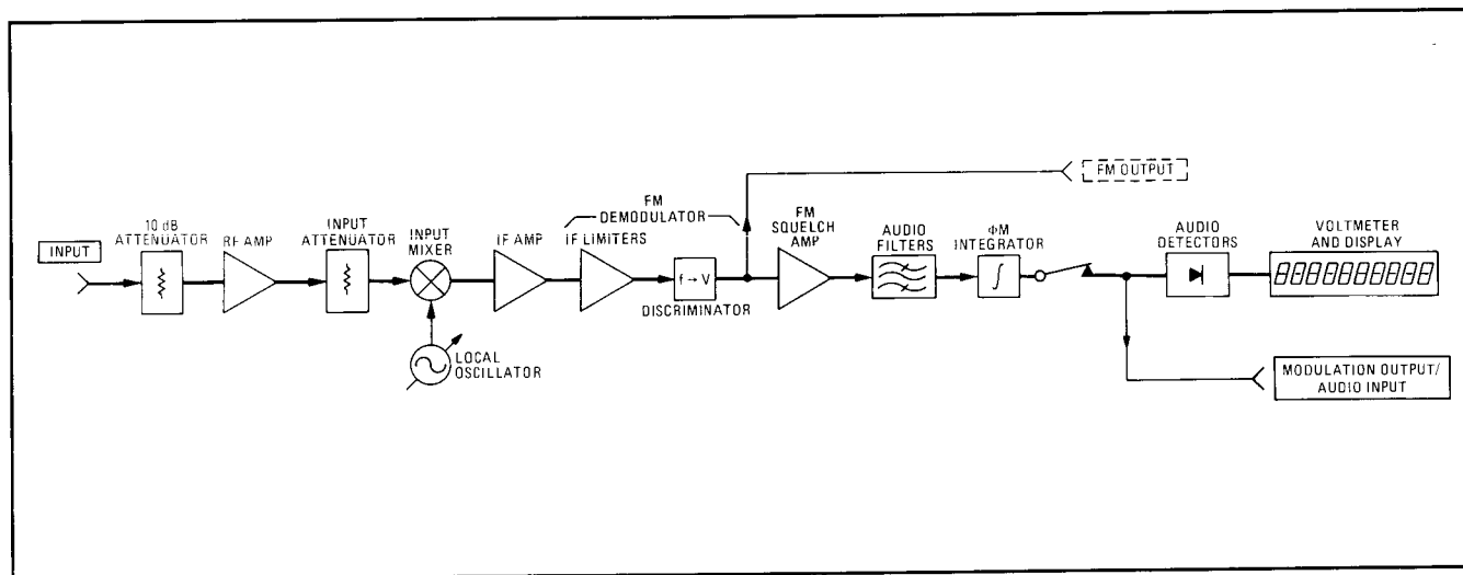
\Phi M Measurement Block Diagram
