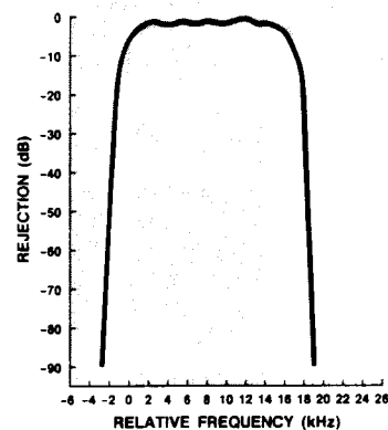
25 kHz Filter Shape (Option 033)
