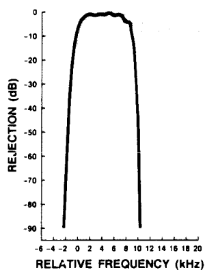
12.5 kHz Filter Shape (Option 032)
