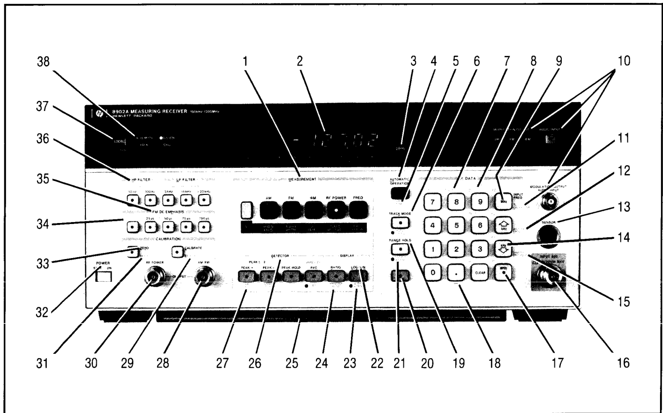
Figure 3-1. Front-Panel Features
