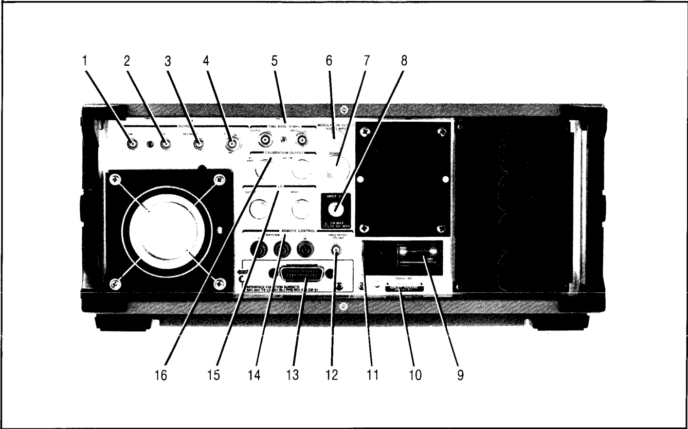
Figure 3-2. Rear-Panel Features
