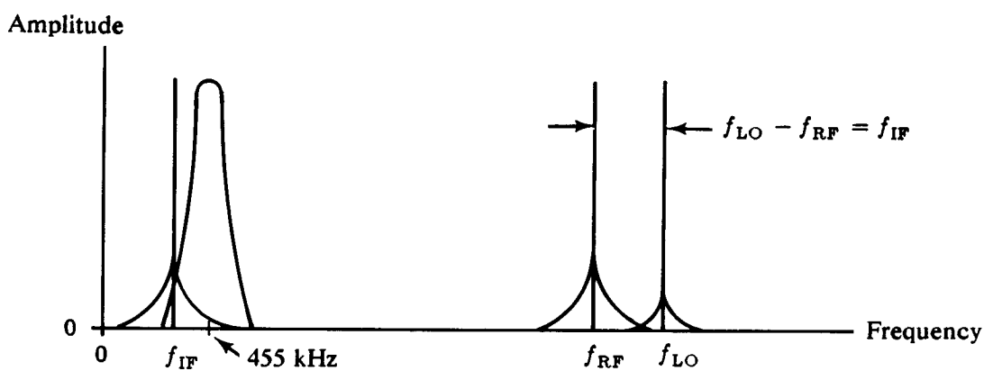
(b.) Frequency Offset by Increasing RF Signal Frequency
