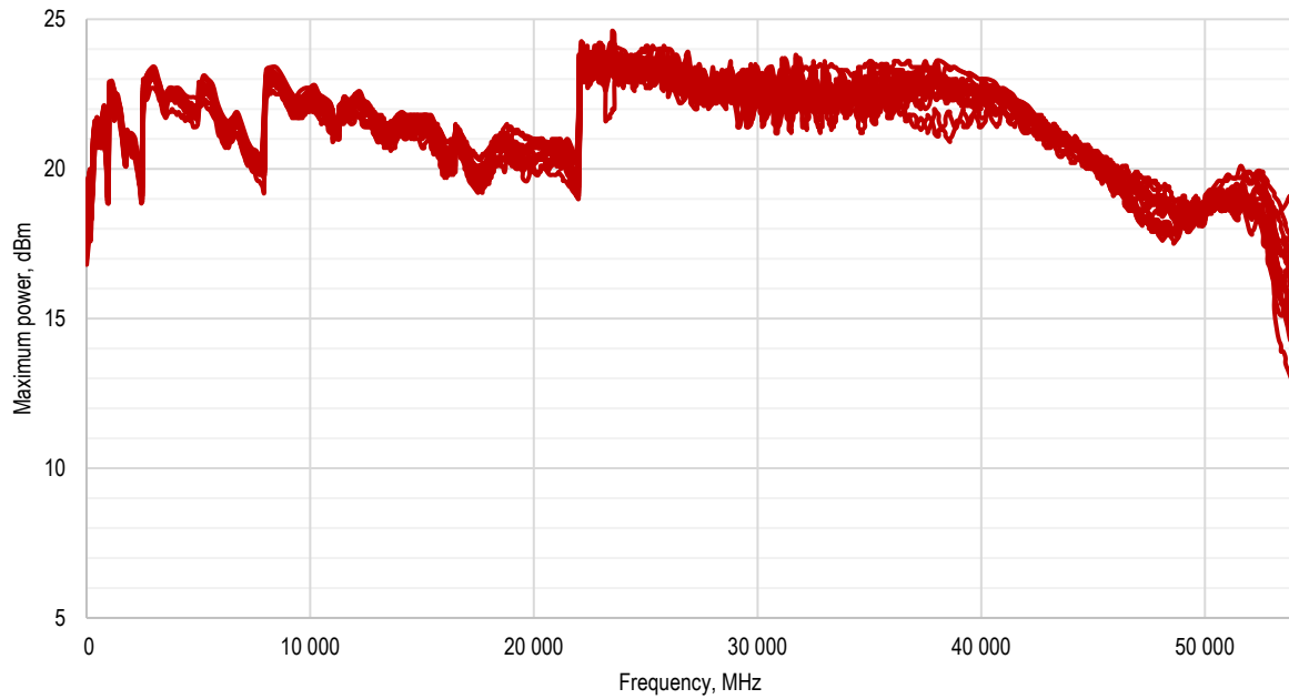
Figure 6. Measured maximum output power, 10 MHz to 54 GHz
