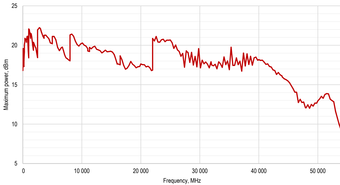
Figure 7. Measured maximum output power, 10 MHz to 54 GHz (Option 2E1)
