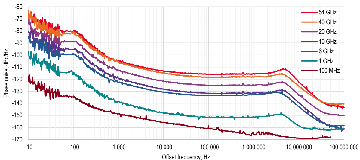
Figure 2. Phase noise at different frequencies, Option LN2 power +10 dBm.
