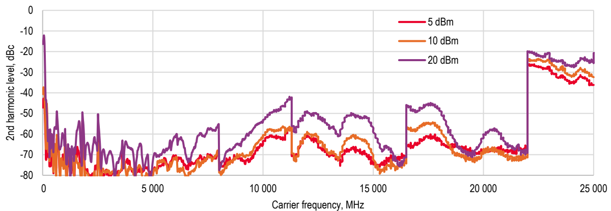
Figure 4. 2 nd Harmonic at different output power
