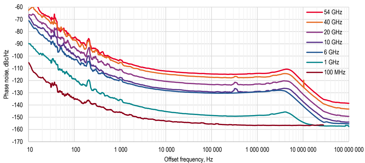
Figure 1. Phase noise at different frequencies, Option LN1 power +10 dBm
