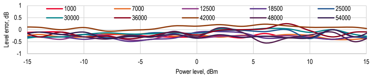
Figure 9. Absolute power level error at different frequencies (Option 554)
