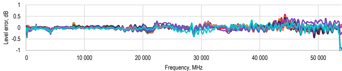
Figure 8. Absolute power level error between -15 and +15 dBm over frequency (Option 554)
