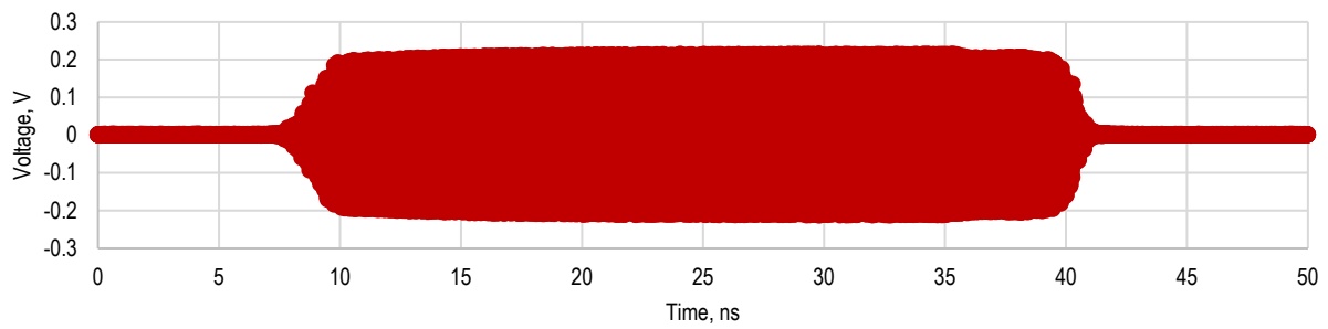
Figure 12. 10 GHz pulse-modulated
