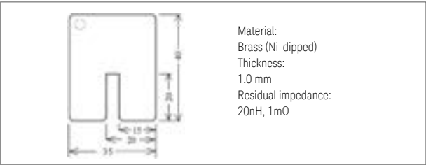
Shorting plate
